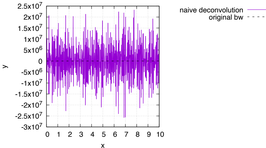
deconvolved breit wigner signal
